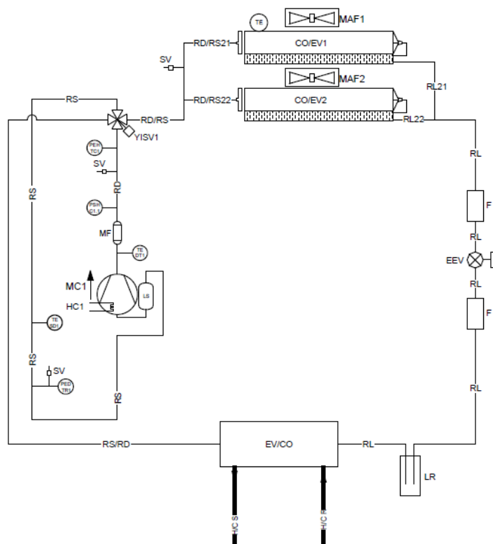
Schema circuito XAIR - PRO 14M-14T-16M-16T- 18T
