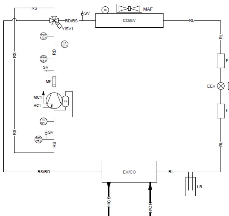
Schema circuito XAIR - PRO 06A-08A-10M-12M- 10T-12T
